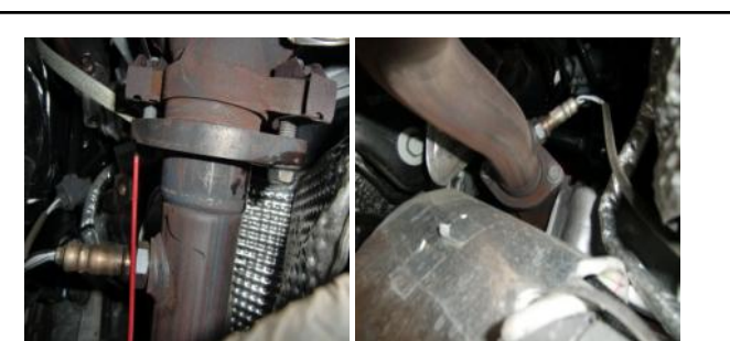
16. On passengers side, unbolt the header from the exhaust. Use some type of thread lubricant to help free rusted exhaust.
