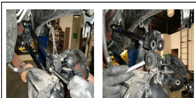
13. Unbolt drivers side front upper arm at the axle.
