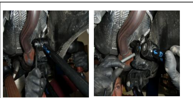
14. Unbolt drivers side front upper arm from the frame.
