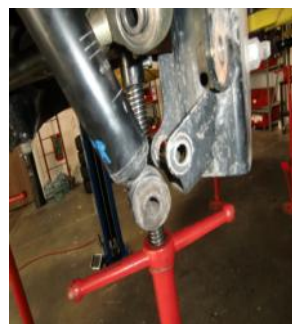
32. Remove the rear shocks.
