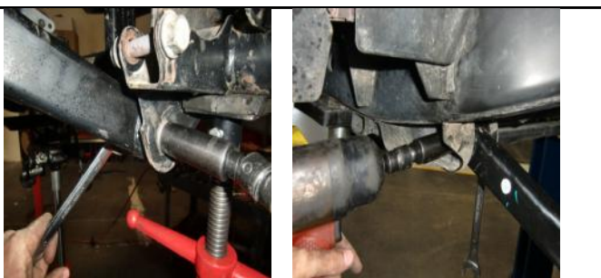
18. Unbolt and remove the both L & R lower arms from the vehicle. Support the differential to prevent axle roll.
