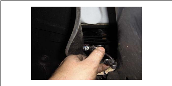
5. Disconnect ABS line at or behind fender liner.
