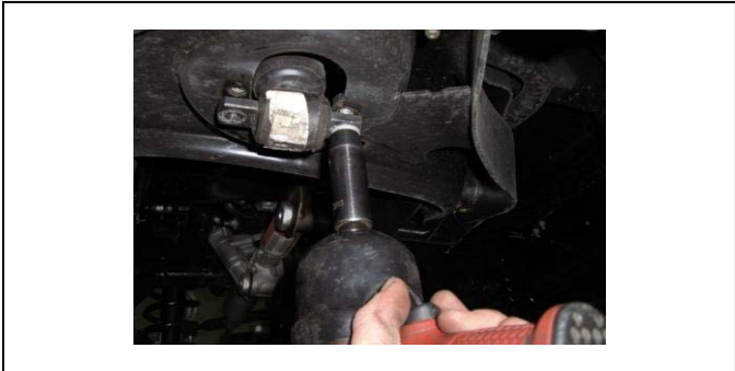
7. Disconnect lower shock mounting bolts.
