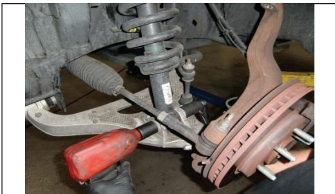
Loosen lower strut bolt/nut and remove.
