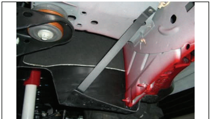
(05-10) Install fender liner strap to clear larger wheel/tires
