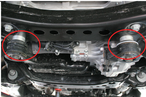
Install (2) differential spacers and tighten to spec
