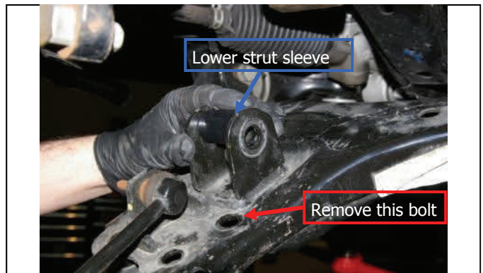
Remove (1) lower ball joint bolt and insert lower strut sleeve
