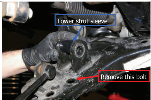
Remove (1) lower ball joint bolt and insert lower strut sleeve
