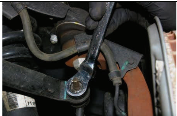
Disconnect and remove sway bar end links
