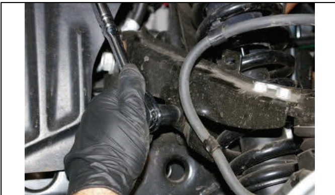
Disconnect brake line bracket from upper control arm
