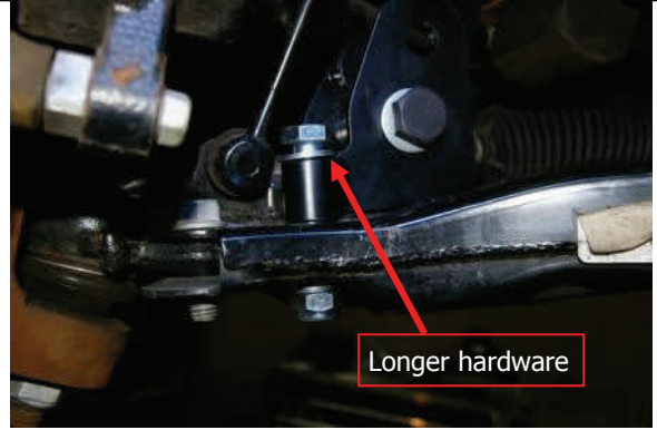
Replace removed lower ball joint bolt with new hardware
