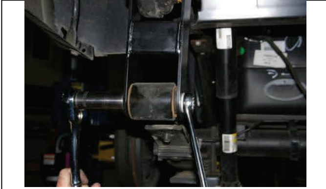
Install new rear lift shackle with OE hardware
