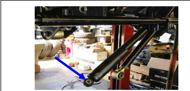
5. Remove the steering damper from the axle.
