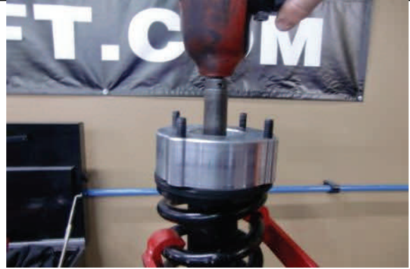
Install new assembled strut extension and tighten to spec.
